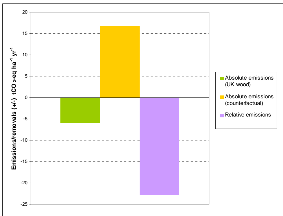
Figure 5.7. Estimation of relative GHG emissions for a characteristic Scottish/UK coniferous forest type for example scenarios involving management for production of wood for a range of materials and fuel (Scenario 23.05, without application of CCS). Absolute emissions are shown for production from Scottish/UK forests, for a counterfactual scenario as well as the resultant relative emissions. Results are shown for 40 year time horizon.
