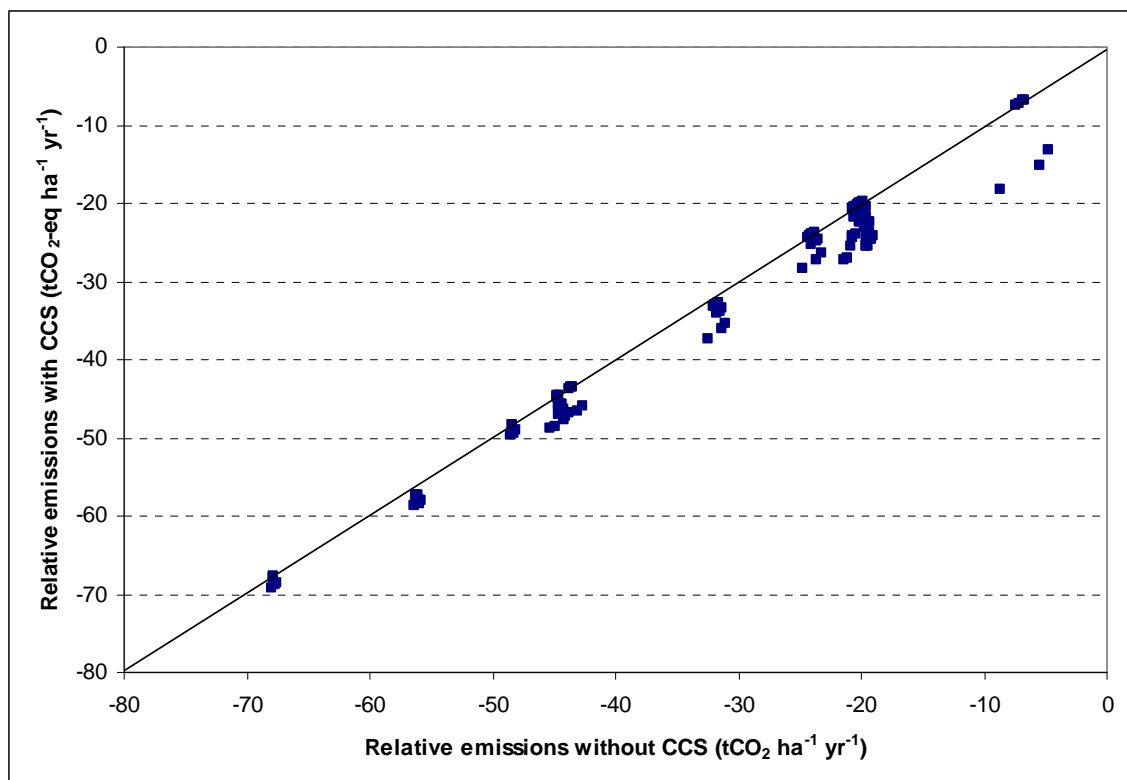
Figure 5.10. Relative greenhouse gas emissions for scenarios involving application of CCS technologies plotted against relative greenhouse gas emissions for equivalent scenarios in which CCS technologies are not applied: Scottish/UK conifer forests managed for production, non-wood counterfactuals, bark utilised for fuel (not mulch), 20 year time horizon. Note that supplementary Scenarios AA and BB are not included.
