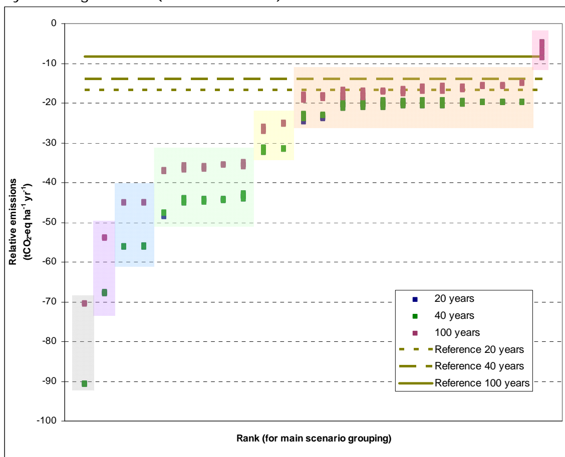
Figure 5.12. Relative greenhouse gas emissions for individual scenarios plotted against rank number for scenario grouping: Scottish/UK conifer forest managed for production, non-wood counterfactuals, bark utilised for fuel (not mulch), CCS not applied, 20, 40 and 100 year time horizons. Note that results for a 20 year time horizon are almost coincident with those for a 40 year time horizon and are obscured. The coloured bands indicate groups of results in terms of similar levels of relative GHG emissions. Note that a scenario grouping based on supplementary Scenario AA is included.
