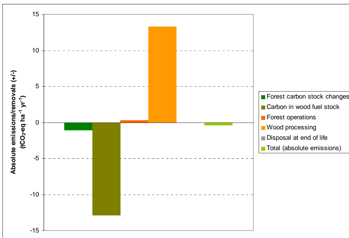
Figure 5.2. Absolute GHG emissions estimated for a characteristic Scottish/UK coniferous forest type for example scenarios involving management for production of wood for fuel only (Scenario 01.06, without application of CCS). Total emissions are shown as well as contributions to the total due to forest carbon stocks, carbon in harvested wood, forest operations and wood processing including combustion. Results are shown for 40 year time horizon.
