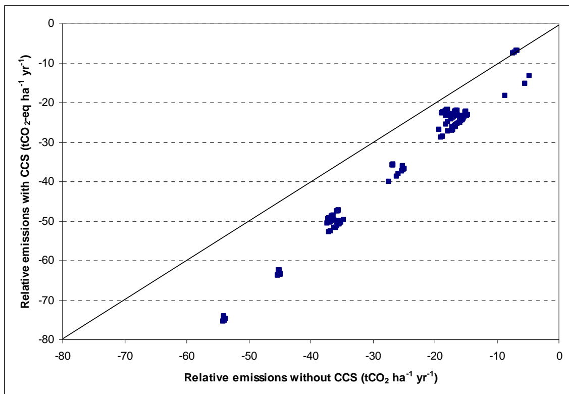
Figure 5.11. Relative greenhouse gas emissions for scenarios involving application of CCS technologies plotted against relative greenhouse gas emissions for equivalent scenarios in which CCS technologies are not applied: Scottish/UK conifer forests managed for production, non-wood counterfactuals, bark utilised for fuel (not mulch), 100 year time horizon. Note that supplementary Scenarios AA and BB are not included.
