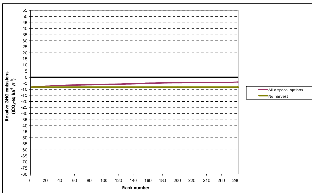
Figure A2.12. Total greenhouse gas emissions plotted against rank number for scenarios involving Scottish/UK conifer forests managed for production: 100 year time horizon, imported wood counterfactuals, CCS applied. Results involving different options for disposal of wood at end-of-life are the same. Note that results for supplementary Scenarios AA and BB are not included.
