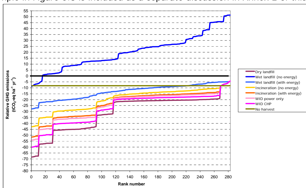
Figure 5.8. Relative greenhouse gas emissions plotted against rank number for scenarios involving Scottish/UK conifer forests managed for production: 100 year time horizon, non-wood counterfactuals, CCS not applied. Results involving different options for disposal of wood at end-of-life are shown separately but may occasionally overlap and obscure each other. Note that results for supplementary Scenarios AA and BB are not included.
