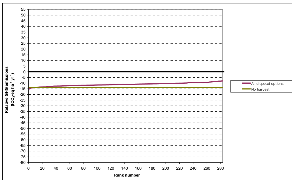
Figure A2.7. Total greenhouse gas emissions plotted against rank number for scenarios involving Scottish/UK conifer forests managed for production: 40 year time horizon, imported wood counterfactuals, CCS not applied. Results involving different options for disposal of wood at end-of-life are the same. Note that results for supplementary Scenarios AA and BB are not included.
