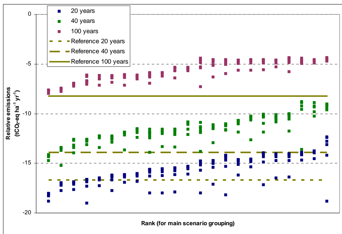
Figure 5.13. Relative greenhouse gas emissions for individual scenarios plotted against rank number for scenario grouping: Scottish/UK conifer forests managed for production, imported-wood counterfactuals, bark utilised for fuel (not mulch), CCS not applied, 20, 40 and 100 year time horizons. The coloured bands indicate groups of results in terms of similar levels of relative GHG emissions. Note that supplementary Scenario AA is not included.
