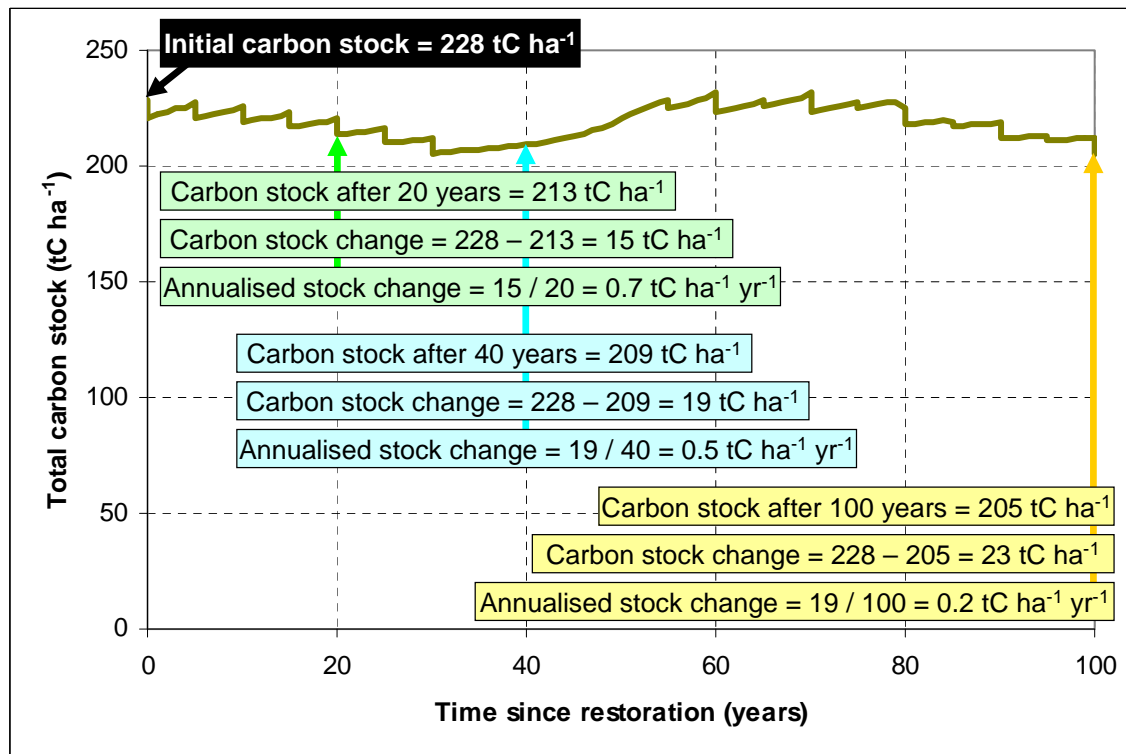
Figure 4.2. Illustration of the calculation of annualised carbon stock changes due to restoration of forest management in ‘neglected’ broadleaf forests.
