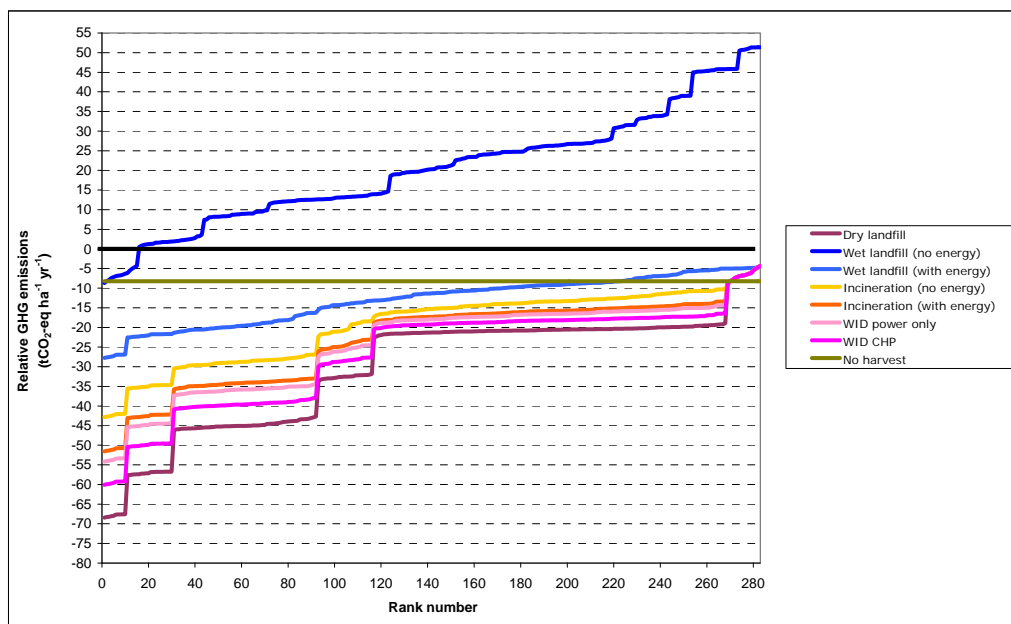
Figure A2.9. Total greenhouse gas emissions plotted against rank number for scenarios involving Scottish/UK conifer forests managed for production: 100 year time horizon, non-wood counterfactuals, CCS not applied. Results involving different options for disposal of wood at end-of-life are shown separately but may overlap and obscure. Note that results for supplementary Scenarios AA and BB are not included.
