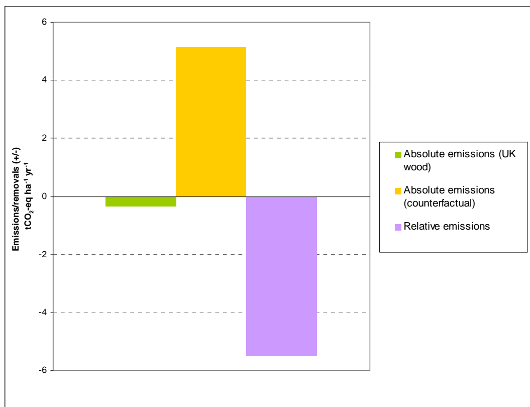
Figure 5.5. Estimation of relative GHG emissions estimated for characteristic Scottish/UK coniferous forest types for example scenarios involving management for production of wood for fuel only (Scenario 01.06, without application of CCS). Absolute emissions are shown for production from UK coniferous forests, for a counterfactual scenario as well as the resultant relative emissions. Results are shown for 40 year time horizon.
