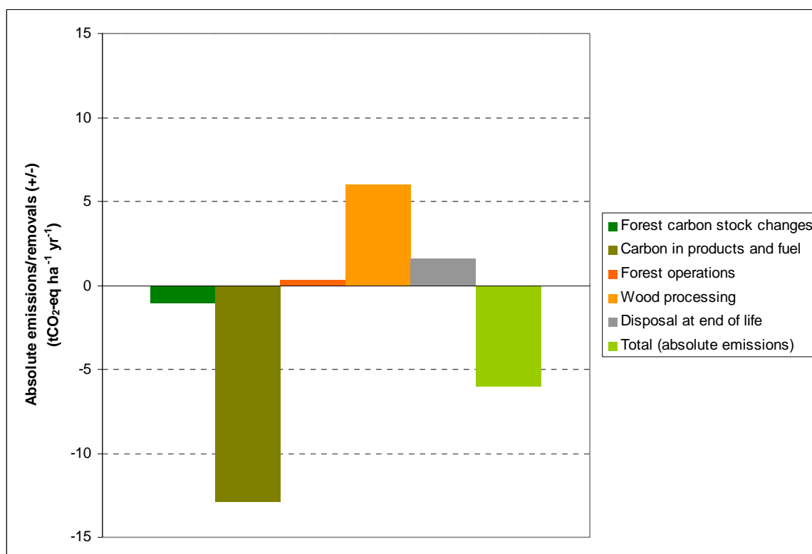
Figure 5.3. Absolute GHG emissions estimated for a characteristic Scottish/UK coniferous forest type for example scenarios involving management for production of wood for a range of materials and fuel (Scenario 23.05, without application of CCS). Total emissions are shown as well as contributions to the total due to forest carbon stocks, carbon in harvested wood, forest operations and wood processing including combustion. Results are shown for 40 year time horizon.
