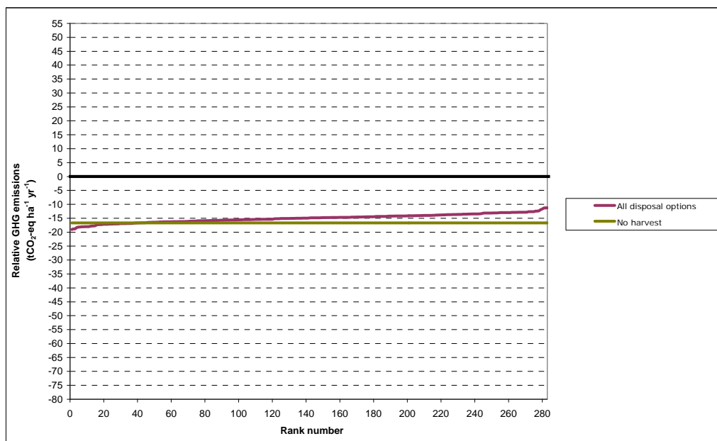
Figure A2.3. Total greenhouse gas emissions plotted against rank number for scenarios involving Scottish/UK conifer forests managed for production: 20 year time horizon, imported wood counterfactuals, CCS not applied. Results involving different options for disposal of wood at end-of-life are the same. Note that results for supplementary Scenarios AA and BB are not included.
