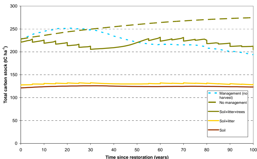
Figure 3.18. Development of carbon stocks over time in trees, litter, soil in a 'neglected' stand of mixed broadleaf trees, where management involving harvesting for timber and biomass production is re-introduced. The results are for a stand of mixed sycamore, ash and birch. The dashed green line shows how carbon stocks in the forest would be expected to continue to accumulate if management was not introduced, in the absence of natural disturbance events. The dashed blue line shows how forest carbon stocks would develop if management was to be introduced involving selective felling of trees and retention of dead wood in the forest to meet environmental and amenity (i.e. non-timber) objectives.
