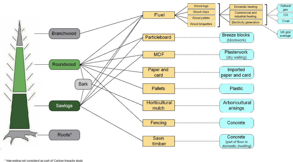
Figure 4.1. Representation of wood harvesting, processing and utilisation chains within this project, including relationships to non-wood counterfactuals. (Note that alternative counterfactuals involving imported wood were also identified and modelled, see Table 4.4.)
