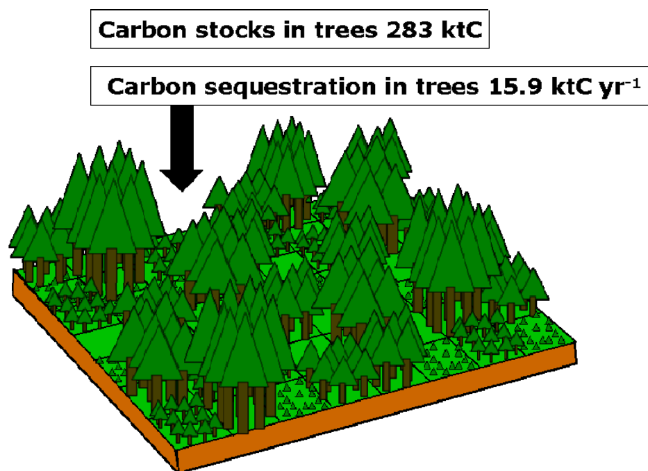
Figure 3.11. Creating a 5,600 hectare forest from even aged Sitka spruce stands over 56 years and resultant impacts on carbon stocks and carbon sequestration: situation after 50 years. (Figure based on the ideas of Piers Maclaren, see Maclaren, 1996, 2000.)
