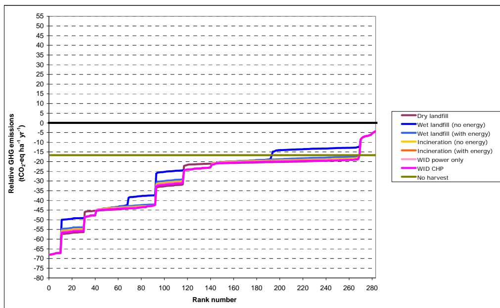
Figure A2.1. Total greenhouse gas emissions plotted against rank number for scenarios involving Scottish/UK conifer forests managed for production: 20 year time horizon, non-wood counterfactuals, CCS not applied. Results involving different options for disposal of wood at end-of-life are shown separately but may overlap and obscure. Note that results for supplementary Scenarios AA and BB are not included.
