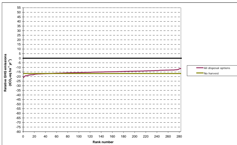
Figure A2.4. Total greenhouse gas emissions plotted against rank number for scenarios involving Scottish/UK conifer forests managed for production: 20 year time horizon, imported wood counterfactuals, CCS applied. Results involving different options for disposal of wood at end-of-life are the same. Note that results for supplementary Scenarios AA and BB are not included.
