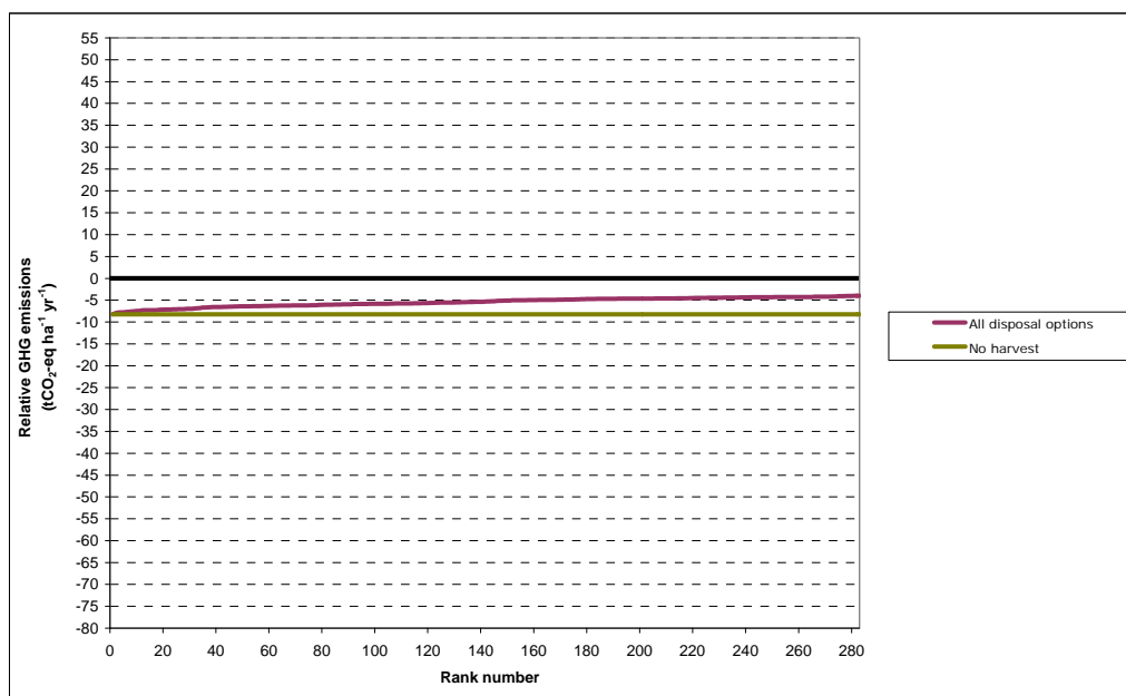
Figure A2.11. Total greenhouse gas emissions plotted against rank number for scenarios involving Scottish/UK conifer forests managed for production: 100 year time horizon, imported wood counterfactuals, CCS not applied. Results involving different options for disposal of wood at end-of-life are the same. Note that results for supplementary Scenarios AA and BB are not included.
