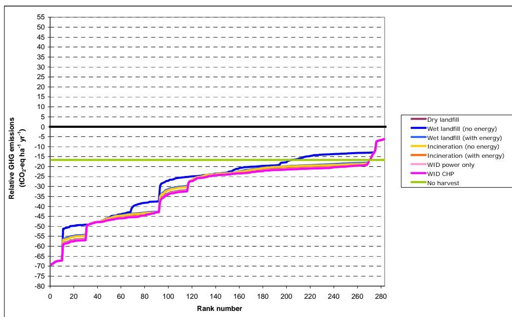
Figure A2.2. Total greenhouse gas emissions plotted against rank number for scenarios involving Scottish/UK conifer forests managed for production: 20 year time horizon, non-wood counterfactuals, CCS applied. Results involving different options for disposal of wood at end-of-life are shown separately but may overlap and obscure. Note that results for supplementary Scenarios AA and BB are not included.
