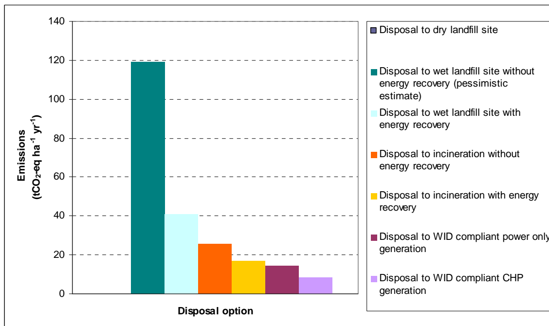
Figure 5.4. Examples of GHG emissions associated with disposal of solid wood products at end-of-life. The results are based on the same scenario as in Figure 5.3 for the characteristic example of Scottish/UK conifer forests managed for production, but the time horizon considered is 100 years. Results are shown for different disposal options. Emissions due to disposal to dry landfill are small and do not register in the graph.
