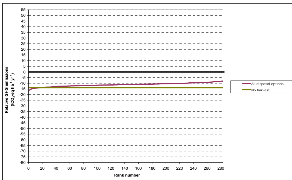
Figure A2.8. Total greenhouse gas emissions plotted against rank number for scenarios involving Scottish/UK conifer forests managed for production: 40 year time horizon, imported wood counterfactuals, CCS applied. Results involving different options for disposal of wood at end-of-life are the same. Note that results for supplementary Scenarios AA and BB are not included.
