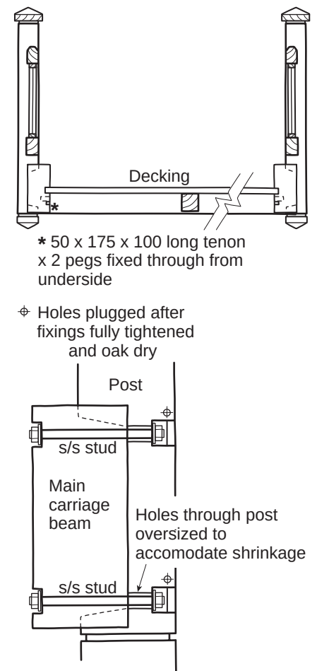
Figure 9.10.3 Parapet connections
