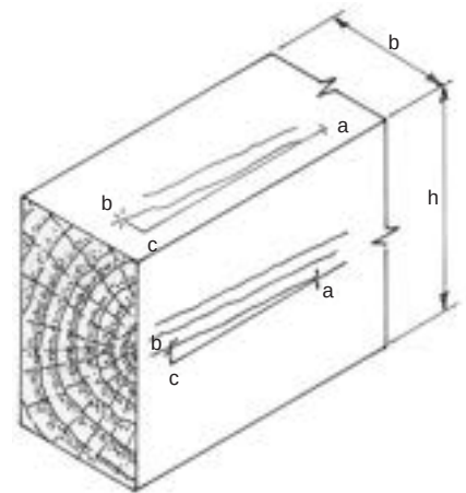
Figure All.10 Slope of grain. Line a – c is imaginary, and parallel to the axis; line a – b is the general grain direction, with irregularities averaged. If a grain scribe is used, line a – b will be marked, perhaps several times. If grain slope is suspected on more than one surface, each should be checked, ie the upper and lateral surface in this Figure
