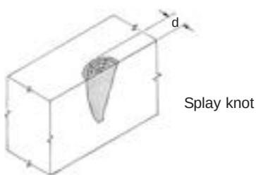
Aris knot d: greater of ( x+z/2 ) or ( z+x/2 )
