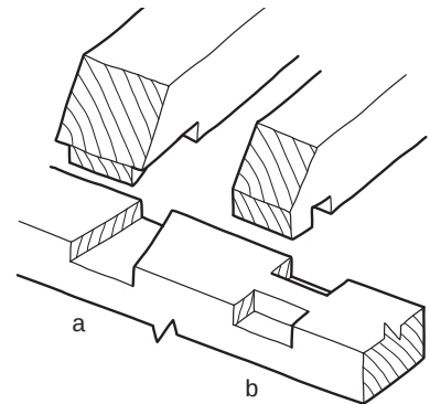
Figure 5.27 Tie beams: a Dovetail b Cog
