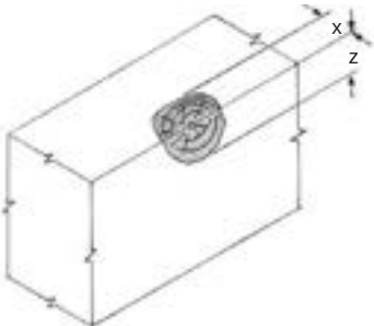
Figure AII.6 Arris knot in a bending member
