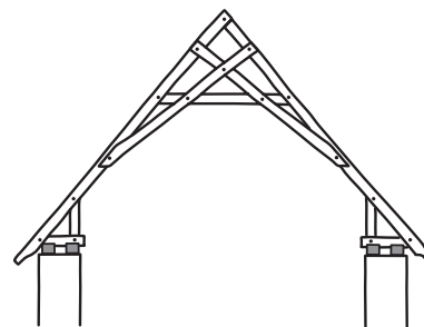
Figure 5.17 Scissors brace
