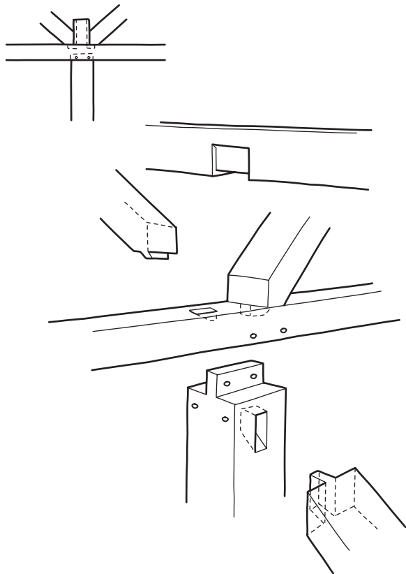
Principal truss: Junction of topmost purlin/upper collar
