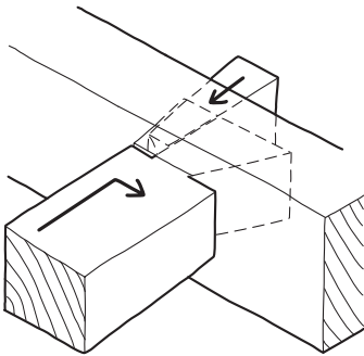
Figure 5.25 Wedged dovetail tenon
