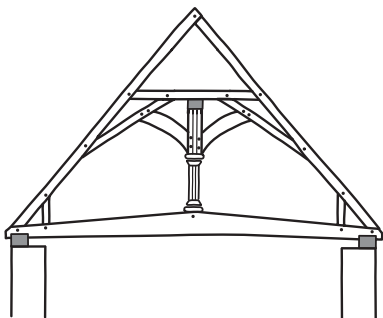
Figure 5.18 Crown post
