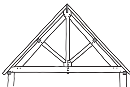
Figure 5.35 King post truss
