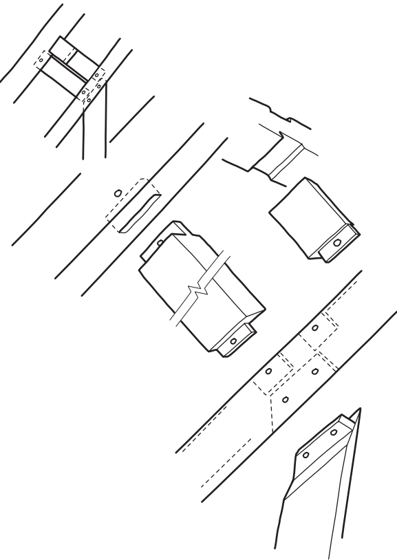
Junction of rafters / lower purlin / hammer post
