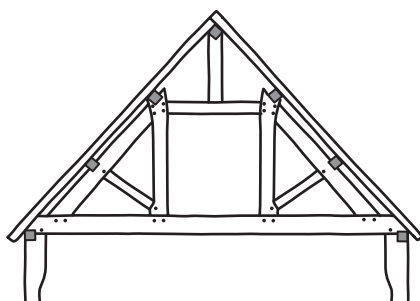
Figure 5.36 Queen post truss
