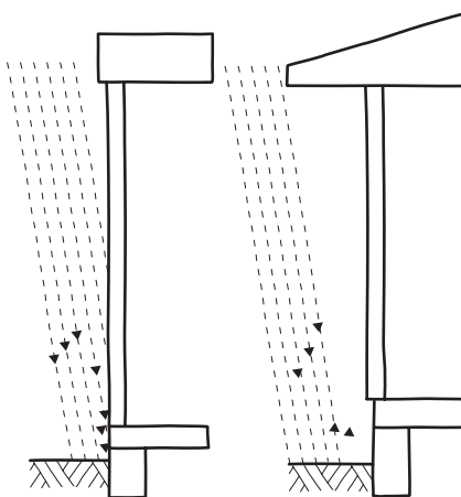
Figure 8.9 Protection afforded by roof overhangs; avoid extending timber cladding into splash zones
