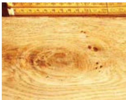
Figure 6.19 A cluster of pin knots around a single main knot, the “cat’s paw”- some caution is needed in grading this feature
