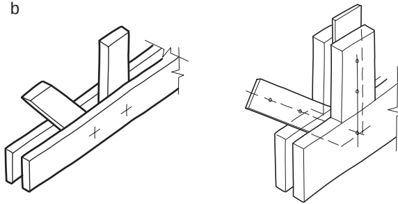
Figure 5.40 Flitch plate joint
