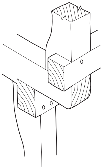
Figure 5.32 Jetty assembly
