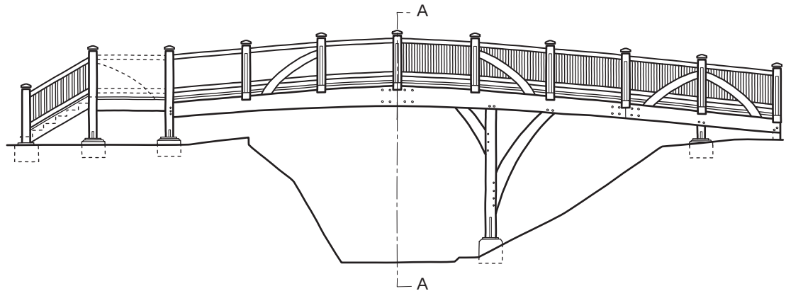
Figure 9.11.2 Bridge elevation
